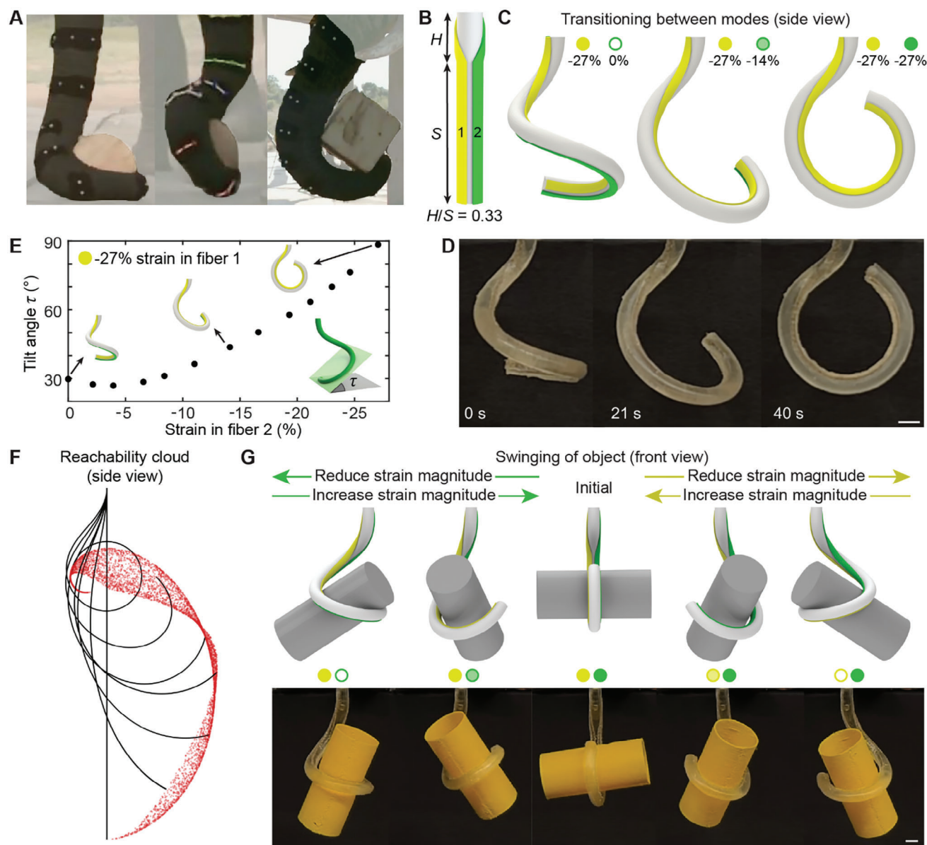
Figure 4. Tunable deformation of the robotic arm by fiber contraction. A) Images of an elephant trunk grasping various objects (Adapted with permission, CC-BY. [6b] ). The trunk can reorient its bending to grasp each object. B) Schematic of the 2-fiber robotic arm design, with H/S = 0.33 , \alpha = 12.59^\circ . The LCE fibers are denoted as fiber 1 (yellow) and fiber 2 (green). C) FEA and D) experimental results of the robotic arm transitioning from coupled bending and twisting modes to a pure bending mode. The circles denote the actuated fiber, with fiber 1 actuated at a constant strain of -27\% and fiber 2 gradually changed from 0\% to -27\% strain. E) Tilt angle, \tau , versus strain of fiber 2 from FEA while fiber 1 is held constant at -27\% strain. F) Theoretical prediction from the AF model of the cloud of reachable points for the tip of the robotic arm under different combinations of contraction in each fiber, with a maximum deformed fiber strain of -33\% . G) Demonstration via FEA (top) and experiment (bottom) of the arm lifting an object and swinging it from right to left by varying the strain in each fiber. The object is adhered to the robotic arm. Scale bars: 4 mm.
